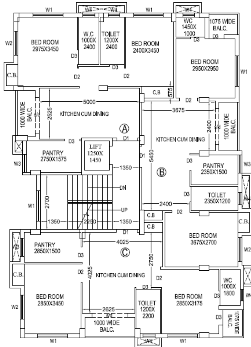
1ST TO 4TH FLOOR PLAN
